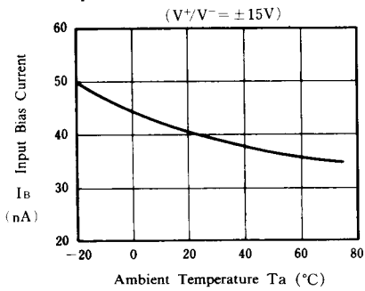
Input Bias Current vs. Ambient
