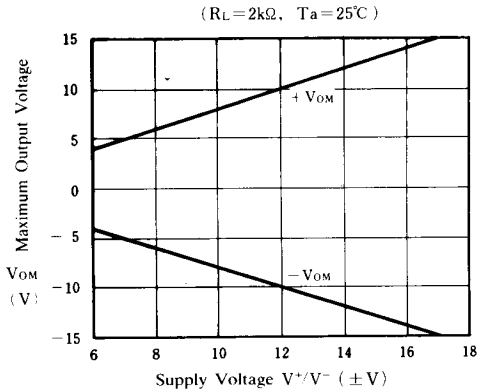
Maximum Output Voltage Swing vs. Supply Voltage
